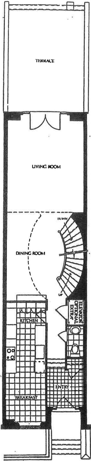
MAIN FLOOR
